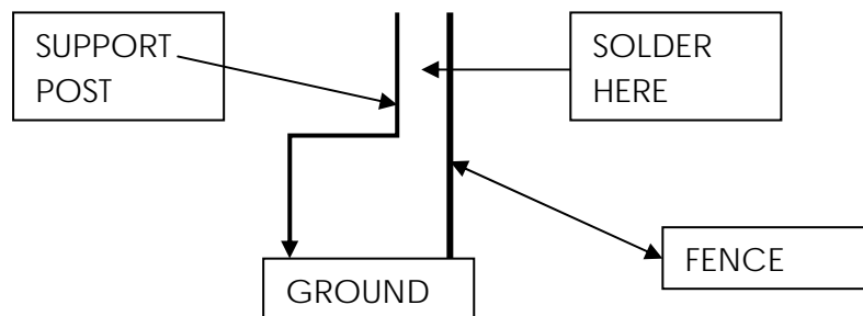
Figure 3. Corner post diagram to support the fence. □
